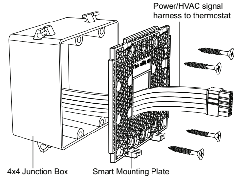
Figure 1. Assembly, exploded view
