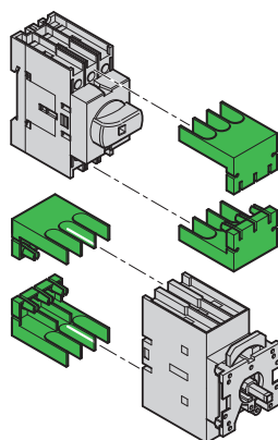
Figure 4: Terminal covers
