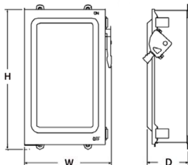
200 A Enclosed Switch Dimensions
