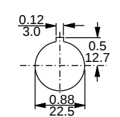
Single-Hole Mounting Dimensions
