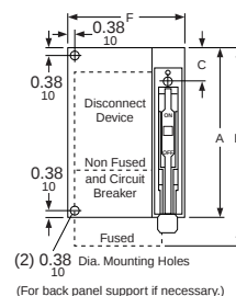
Switch Type Maximum Voltage Fuse Type Dimension A Dimension B 30 A 30 A, 250 V H, K, R 1.625 — 30 A, 600 V H, K, R 4.25 30 A, 600 V J 1.625 60 A 60 A, 250 V H, K, R 2.25 60 A, 600 V H, K, R 4.75 60 A, 600 V J 1.625 100 A 100 A, 250 V H, K, R — 3.25 100 A, 600 V H, K, R 5.25 100 A, 600 V J 3.25
