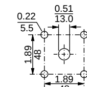
Four-Hole 60 x 60 Mounting Dimensions [9]
