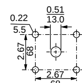
Four-Hole 90 x 90 Mounting Dimensions [9]
