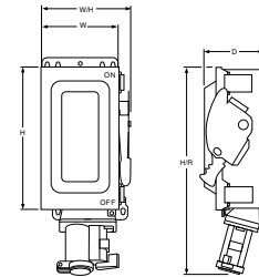
Crouse-Hinds Receptacle
