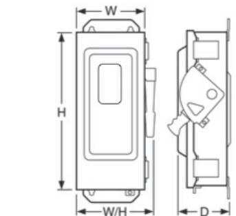
Typical 30-200 A Type 4, 4X, 5, 12 Enclosure (Stainless has flat front)
