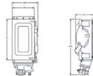
Appleton Receptacle
