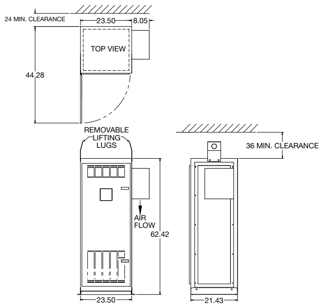
Figure 1—AV4000
