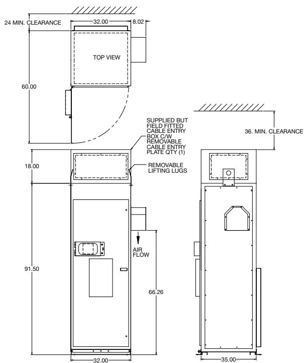
Figure 3—AT6000
