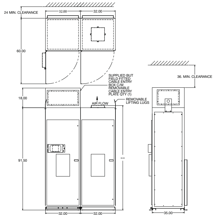
Figure 4—AT6000 (2 Section)
