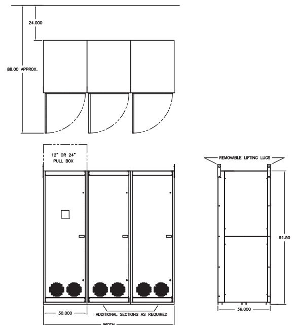
Figure 2—AV5000 and 6000
