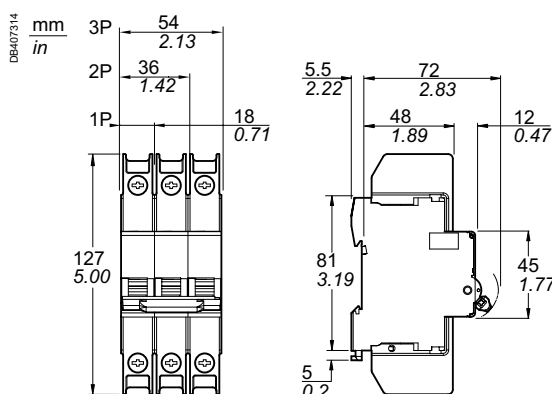
C60BPR Ring tongue terminal
