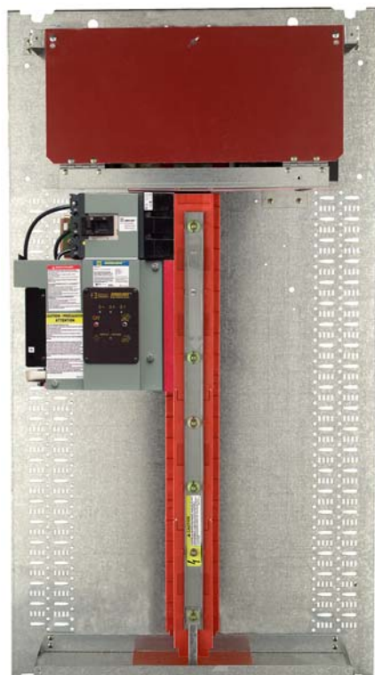
I-Line Plug-On Unit with SurgeLogic SPD
