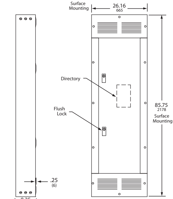
Typical 2-Piece Trim with Optional Door
