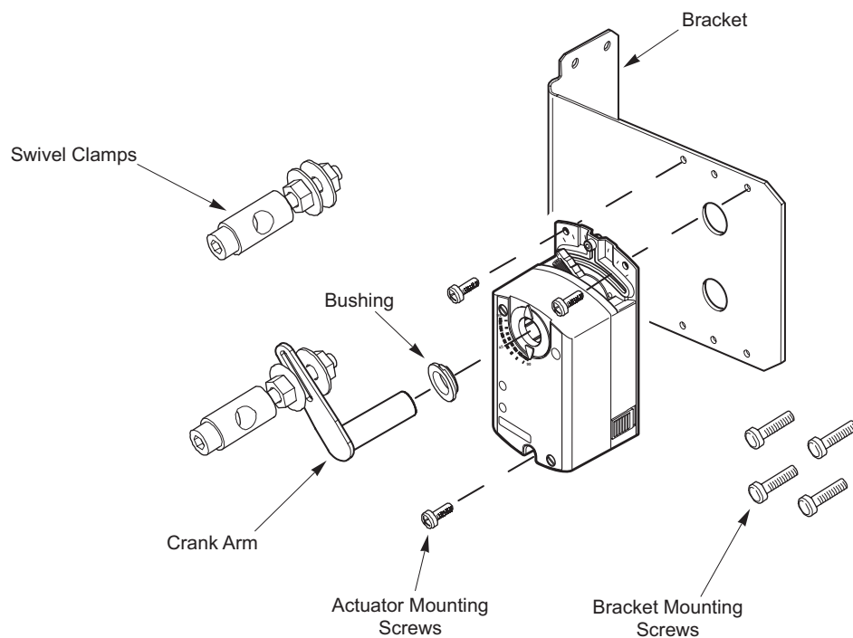
Figure-2 Installation of AM-726 Accessory Kit.
