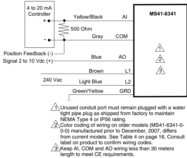
Figure-6 Typical Wiring Diagram for a 4 to 20 mA Controller with a 240 Vac Actuator.
