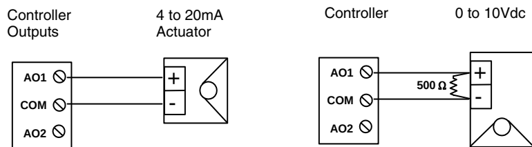
Figure-5 Analog Output Connections for 4 to 20mA and 0 to 10Vdc Actuators.
