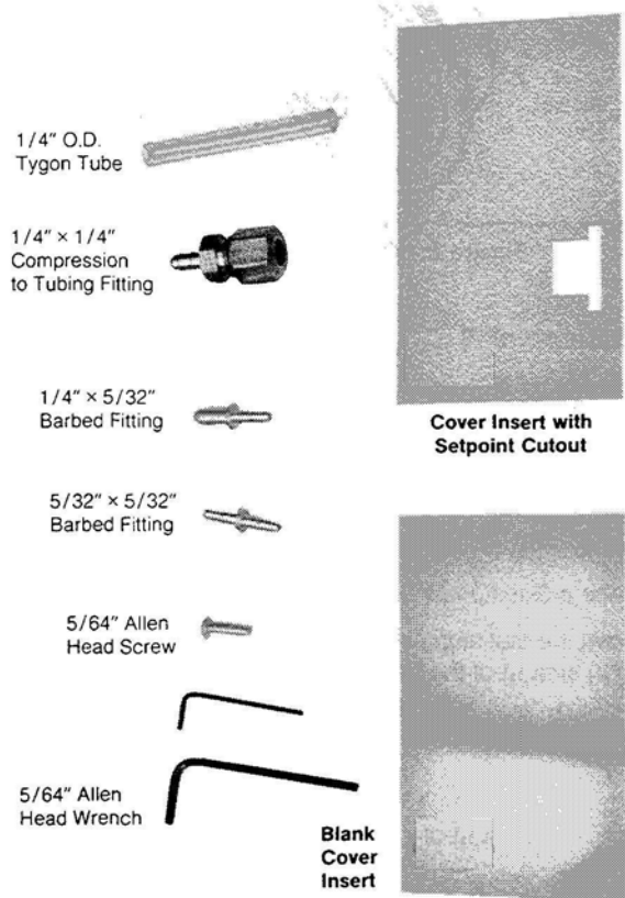
Figure-1 Part Identification.
