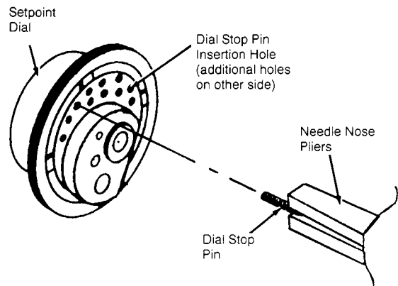
Figure-3 Dial Stop Pin Insertion.
