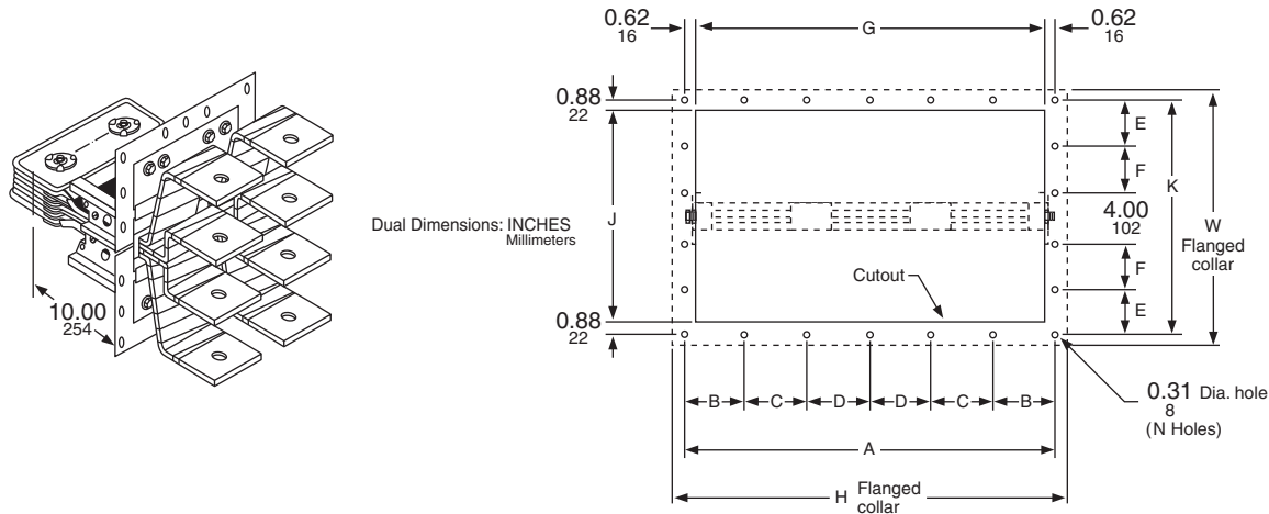
Figure 73: Flanged End: Catalog Number Suffix-10FEB Dimensions
