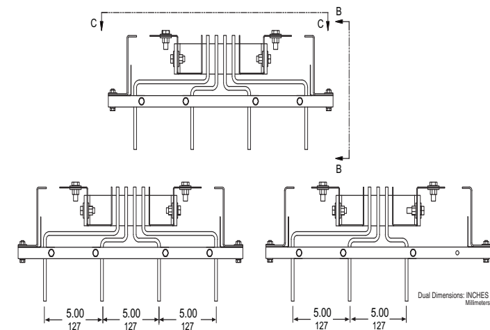
Figure 72: New Qwik Flange Dimensions
