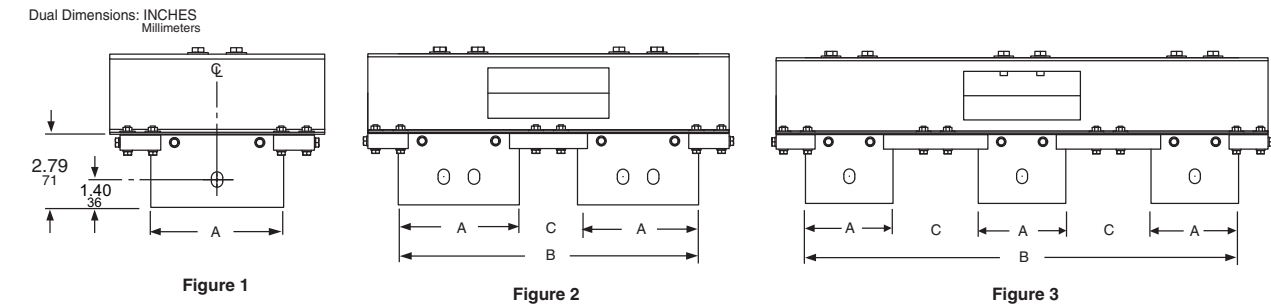
Figure 71: New Aluminum and Copper Qwik Flange (Indoor Only) Dimensions
