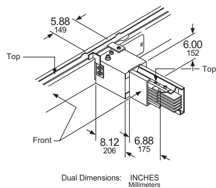
Figure 39: Tees
