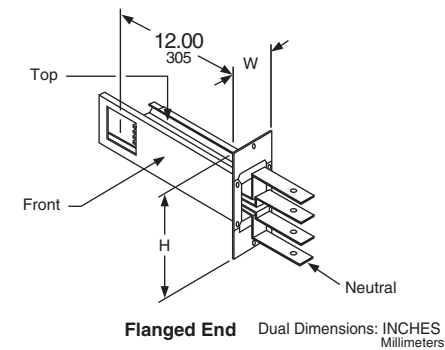
Figure 46: Catalog Number Suffix–FES 12 (Slot End) / FEB 12 (Bolt End)
