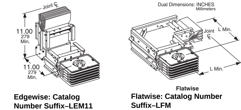
Figure 77: Elbows
