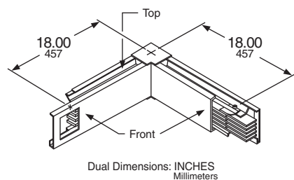
Figure 42: Front Inside Elbow: Catalog Number Suffix-LFI
