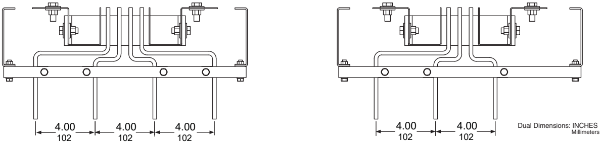
Figure 69: Legacy Qwik Flange Dimensions
