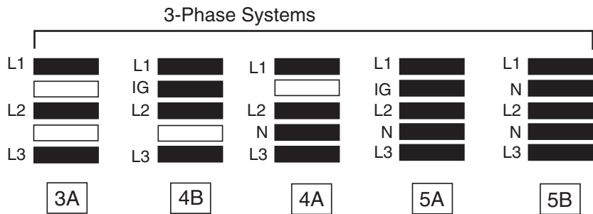
Figure 130: Busbar Configuration
