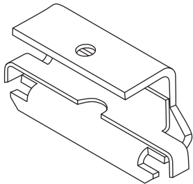
Figure 50: Flatwise Hanger
