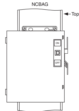
Figure 25: Correct Orientation of Riser Busway
