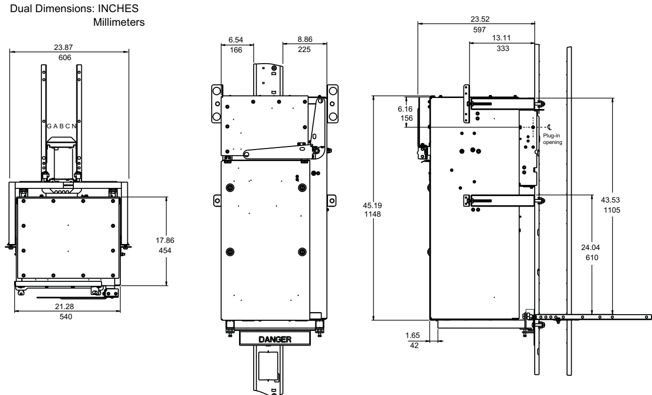
Figure 120: Fusible Switch Bolt-On Units (Vertically Mounted)
