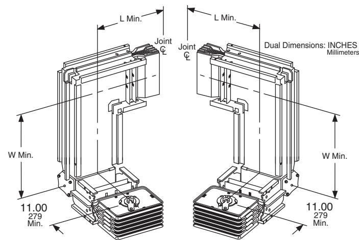
Figure 79: Double Elbows
