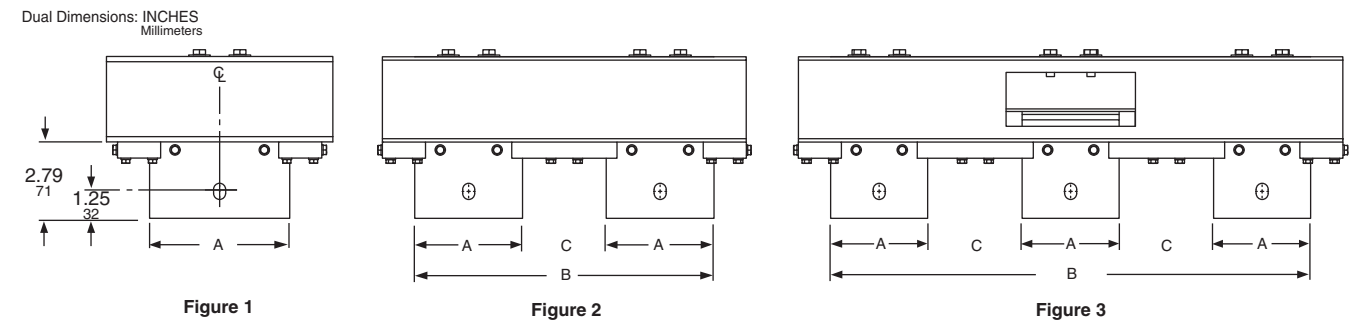
Figure 68: Legacy Aluminum and Copper Qwik Flange Dimensions
