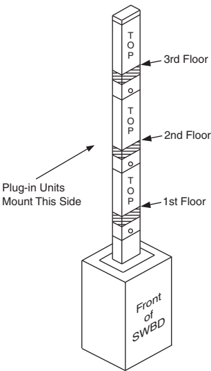
Figure 12: Plug-In Riser Fed by Switchboard
