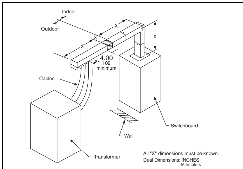
Figure 18: Transformer Tap for One Three-Phase Transformer
