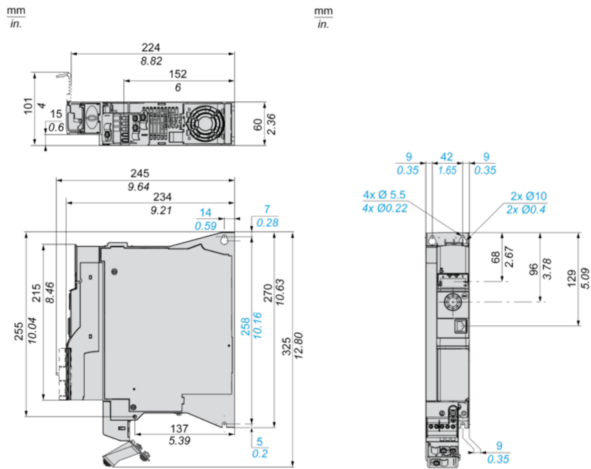
Bottom, Right and Front View
